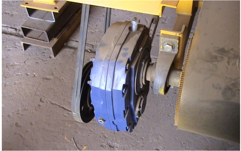
Conveyor Belt Drive
